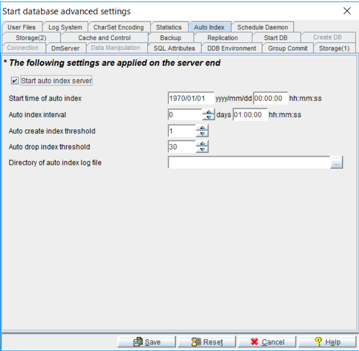
Figure 4-11 Auto Index page of the Start Database Advanced Settings window
