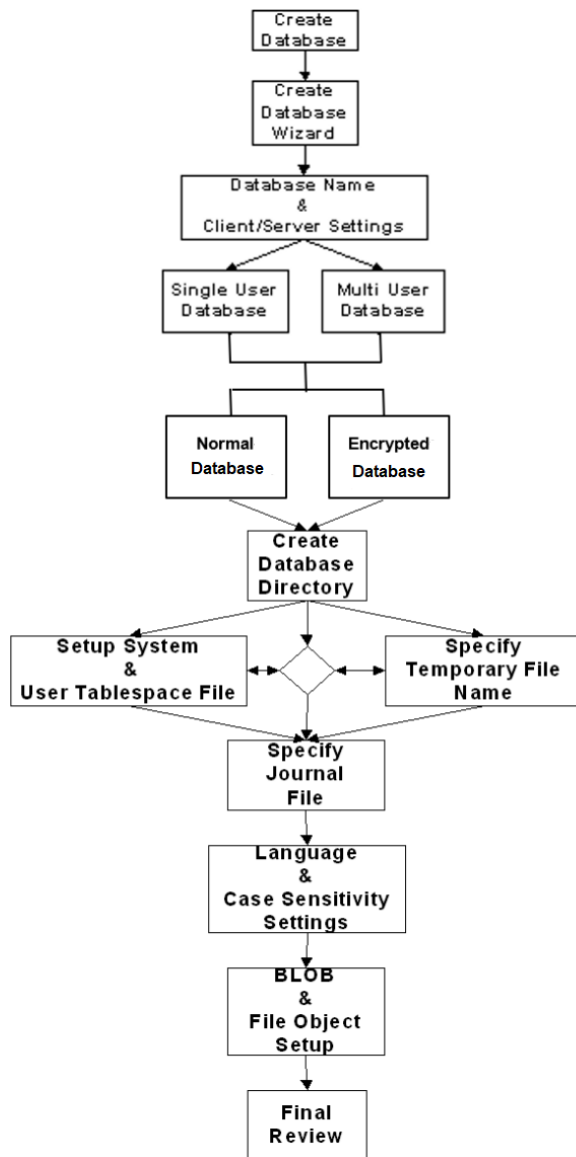
Figure 3-6 Program Logic for the Create Database Wizard
