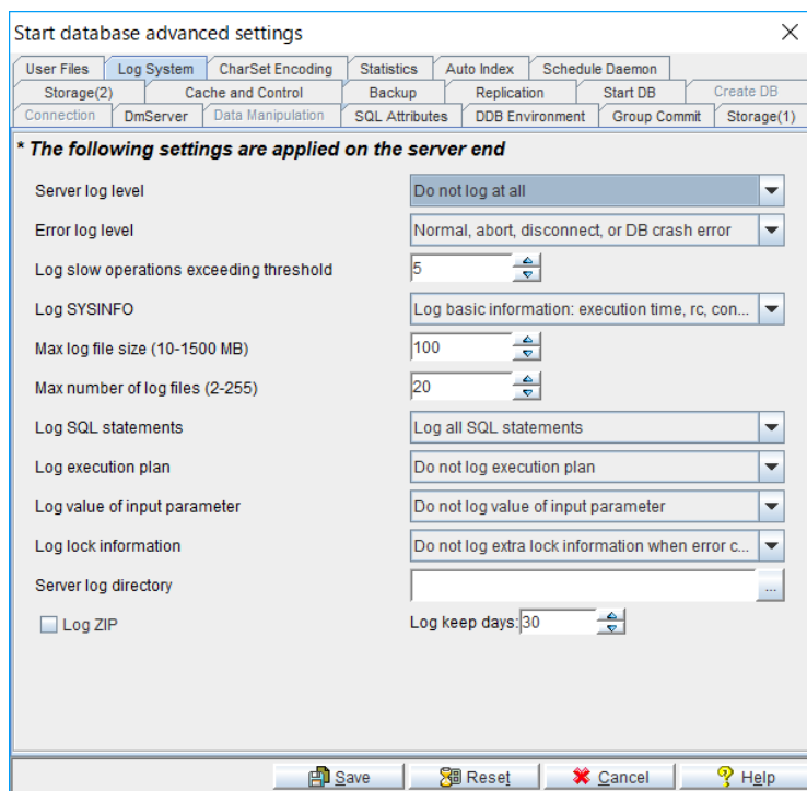
Figure 4-8 Log System page of the Start Database Advanced Settings window
