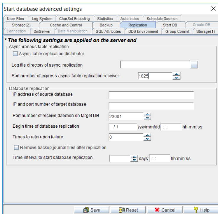
Figure 4-2 Replication page of the Start Database Advanced Settings window
