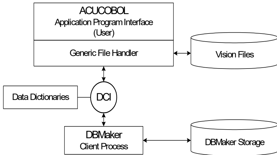
Figure 2-3 Data Flowchart
