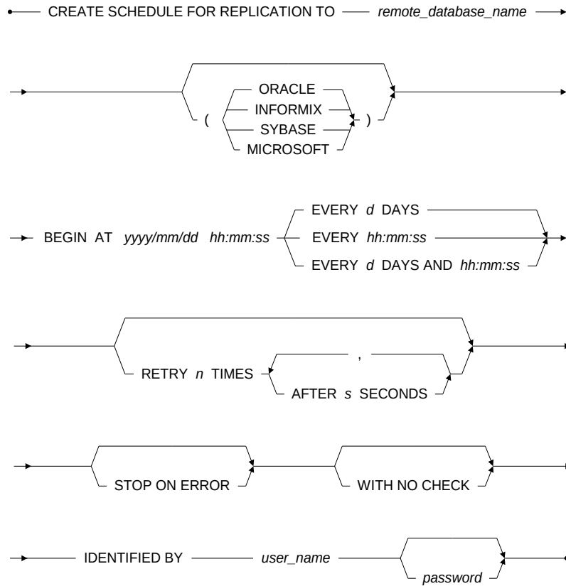
Figure 17-6 Syntax for the CREATE SCHEDULE Statement
