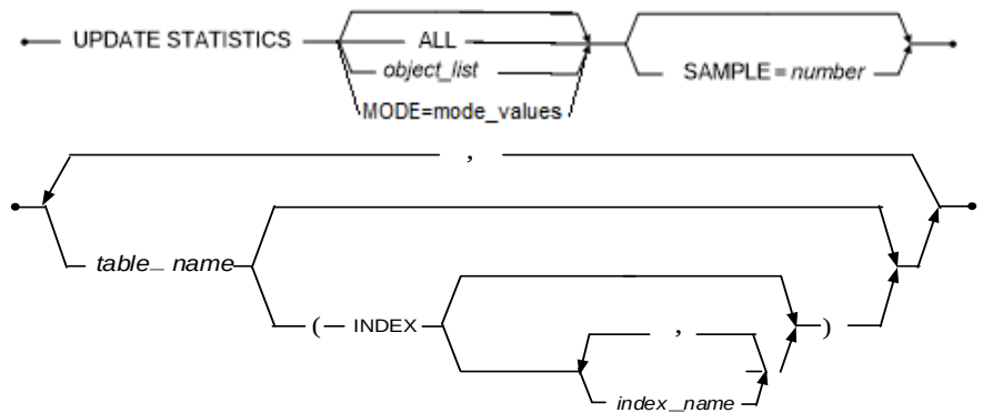
Figure 20-1 Syntax for the UPDATE STATISTICS Statement
