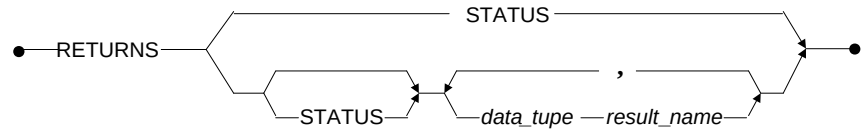
Figure 12-1 Syntax for the CREATE PROCEDURE statement
