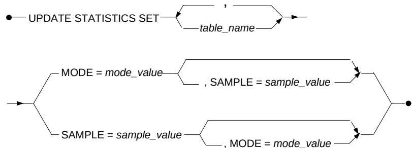
Figure 20-2 Syntax for the UPDATE STATISTICS SET statement
