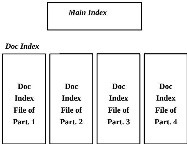
Inverted-File Structure with Four Partitions
