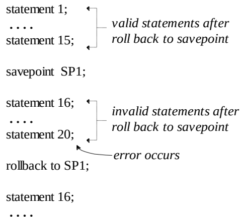
Figure 9-2 Using Savepoints
