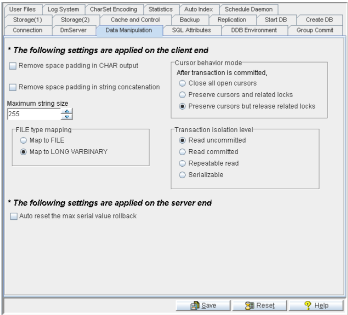
Figure 3-3 Data Manipulation Page
