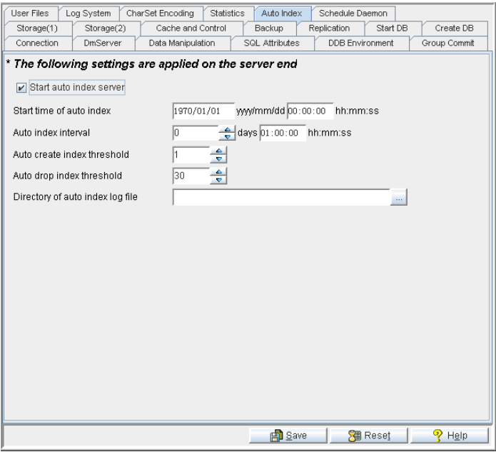
Figure 3-18 Auto Index Page
