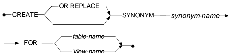
Figure 7-2 Syntax for the CREATE SYNONYM statement
