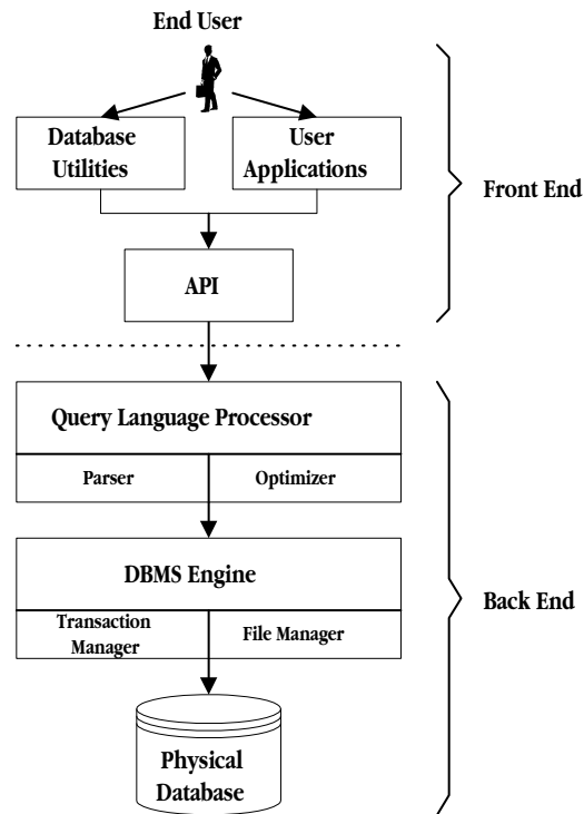
Figure 3-2: Common functions and components of a RDBMS
