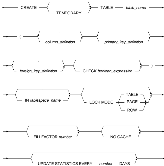
Figure 5-1: Syntax diagram for the CREATE TABLE command
