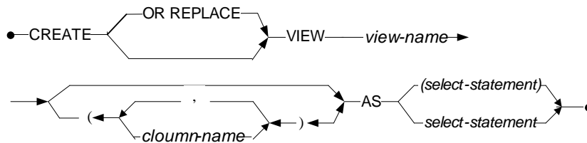
Figure 7-1 Syntax for the CREATE VIEW statement
