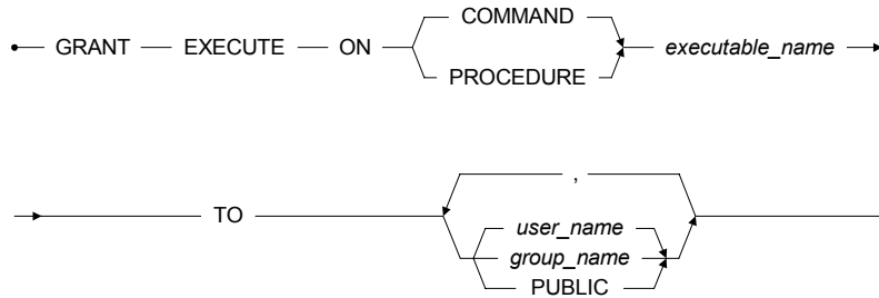
Figure 12-9 Syntax for the GRANT EXECUTE privileges statement
