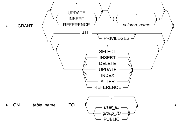
Figure 8-11 Syntax for the GRANT command
