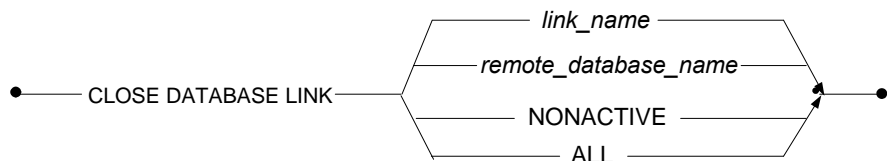
Figure 15-6 Syntax for closing a database link
