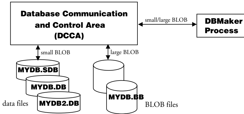
Figure 7-2: DBMaker accesses BLOB data through DCCA
