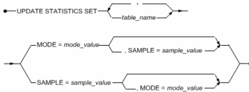
Figure 18-2 Syntax for the UPDATE STATISTICS SET statement
