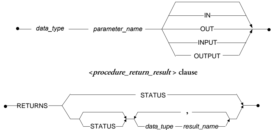
Figure 12-1 Syntax for the CREATE PROCEDURE statement
