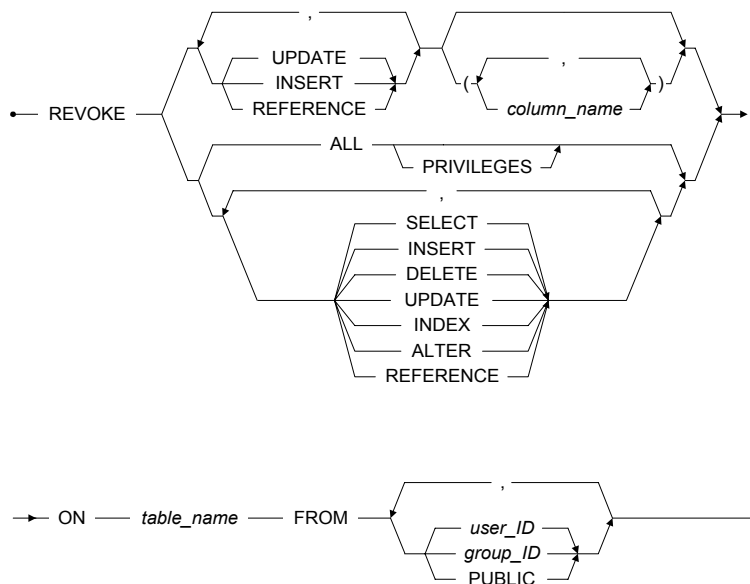
Figure 8-12 The REVOKE (object privileges) command
