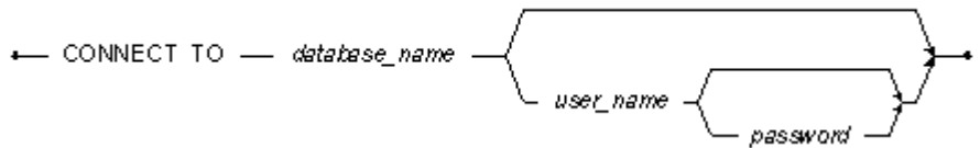
Figure 6-2 CONNECT syntax
