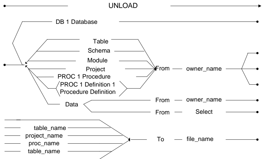
Figure 6-12 UNLOAD syntax
