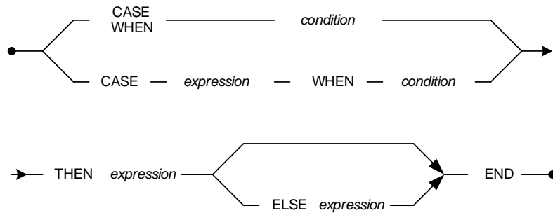
Figure 3-100 CASE Syntax
