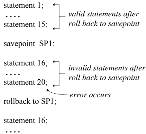
Figure 9-2 Using Savepoints
